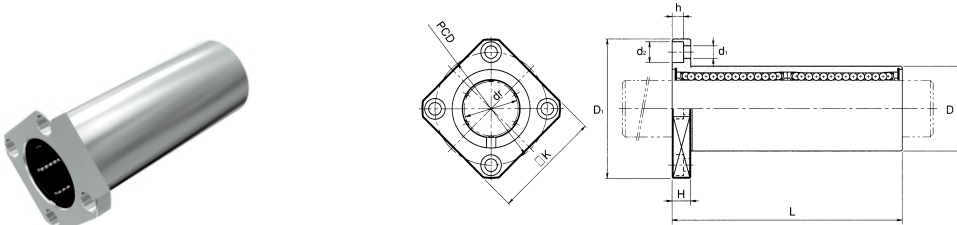
LMK-L/LMK-LM形
