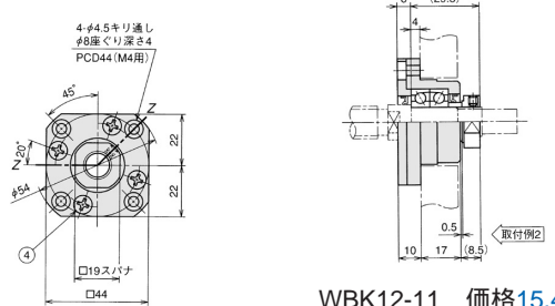
WBK12-11 価格15,400
