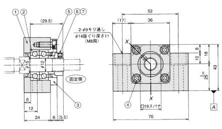
WBK12-01A 価格15,400
