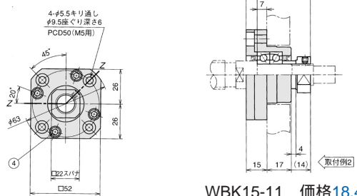
WBK15-11 価格18,400
