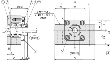
WBK10-01A 価格15,400
