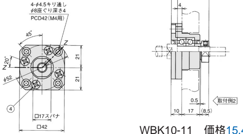
WBK10-11 価格15,400
